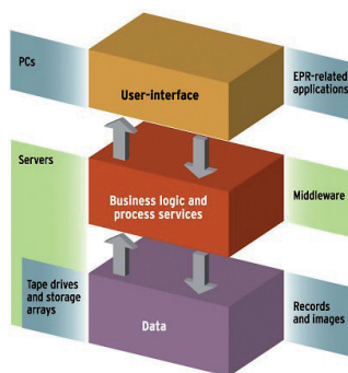
3-tier architecture
